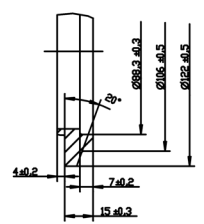
EXHAUST FLANGE 11
