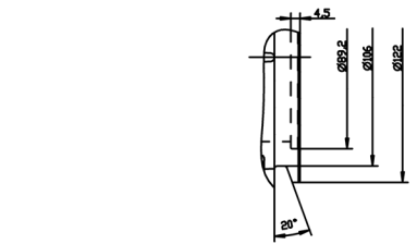
V-CLAMP TURBO CHARGER 11
