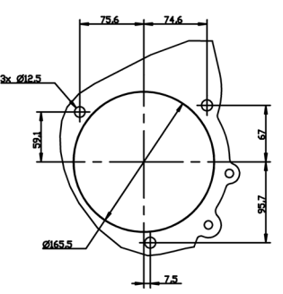
VIEW RR AIR COMPRESSOR PTO 12
