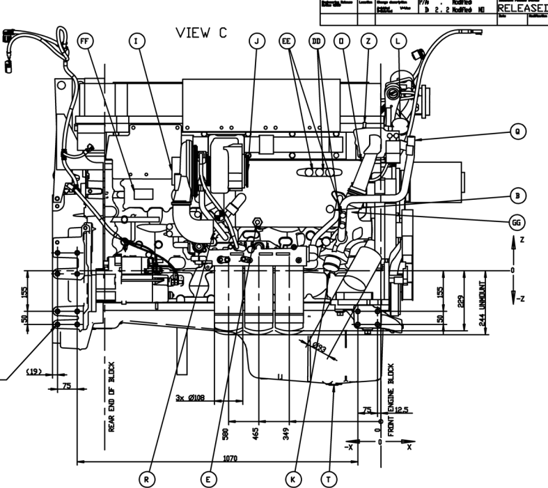
EXHAUST FLANGE 11
