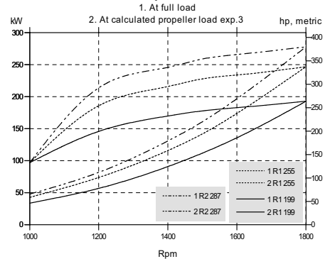
TAMD103A Torque
